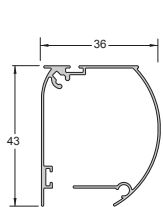
Series 36mm Headbox for smaller openings
